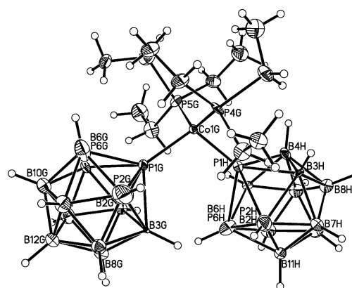
Figure 1. Perspective view of one of four crystallographically independent molecules (molecule GH ) of [HCo(1,2- closo -P 2 B 10 H 10 ) 2 (PEt 3 ) 2 ] ( 1 ). Thermal ellipsoids drawn at 50% probability except for H atoms. There is disorder between P and B atoms in the 5-atom belts to which atoms P1 are connected. Molecule AB : Co1–P1A 2.051(3), Co1–P1B 2.057(3), Co1–P4 2.230(3), Co1–P5 2.179(3) Å. Molecule CD : Co1–P1C 2.072(3), Co1–P1D 2.096(3), Co1–P4 2.194(3), Co1–P5 2.165(3) Å. Molecule EF : Co1–P1E 2.044(3), Co1–P1F 2.038(3), Co1–P4 2.215(3), Co1–P5 2.205(4) Å. Molecule GH : Co1–P1G 2.083(3), Co1–P1H 2.087(3), Co1–P4 2.210(3), Co1–P5 2.207(3) Å.
