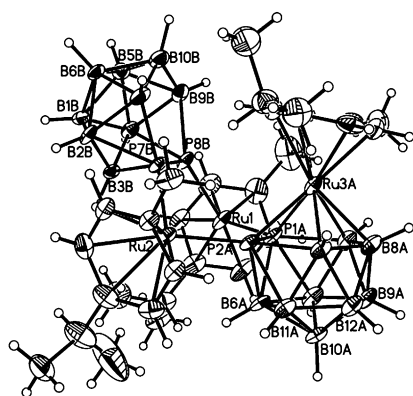
Figure 2. Perspective view of μ-[1,2-{HRu( p -cymene)} 2 -7',8'- nido -P 2 B 9 H 9 ]-3-( p -cymene)-3,1,2- closo -RuP 2 B 9 H 9 ( 2 ). Thermal ellipsoids drawn at 50% probability except for H atoms. Ru1–P1A 2.252(2), Ru1–P8B 2.304(2), Ru2–P2A 2.252(2), Ru2–P7B 2.282(2), Ru3A–P1A 2.371(3), Ru3A–P2A 2.378(3), P1A–P2A 2.348(3), P7B–P8B 2.176(3) Å.
