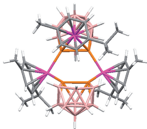
Figure 3. Alternative view of compound 2 looking perpendicular to the Ru3A...B10A axis and showing the approximate C 2 symmetry of the {Ru 3 (P 2 B 9 ) 2 } core. C gray, B pink, P orange, Ru purple, H white.
